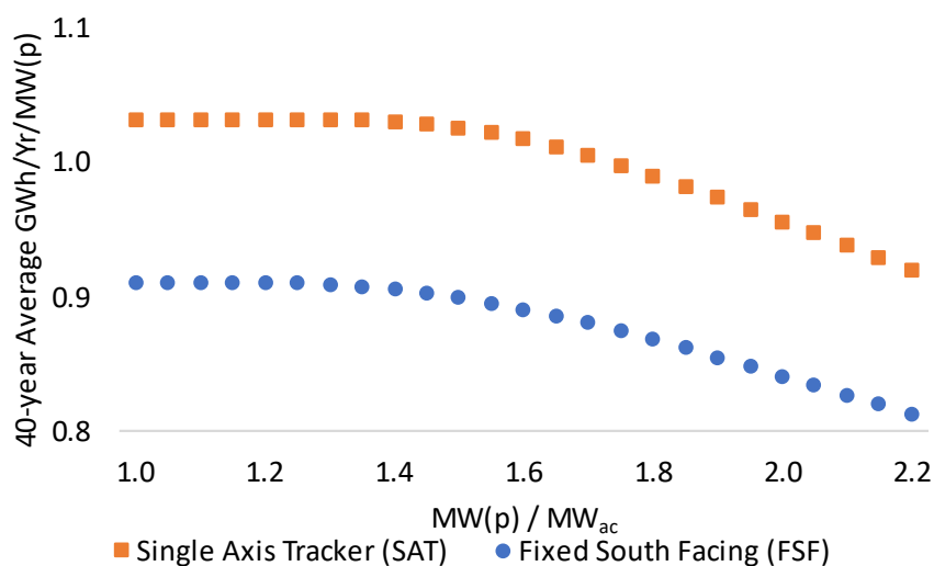
Figure 6-6: GWh/Yr/MW decreases as overplanting increases, and losses are incrementally larger above a ratio of c.1.3. [Author Analysis]
