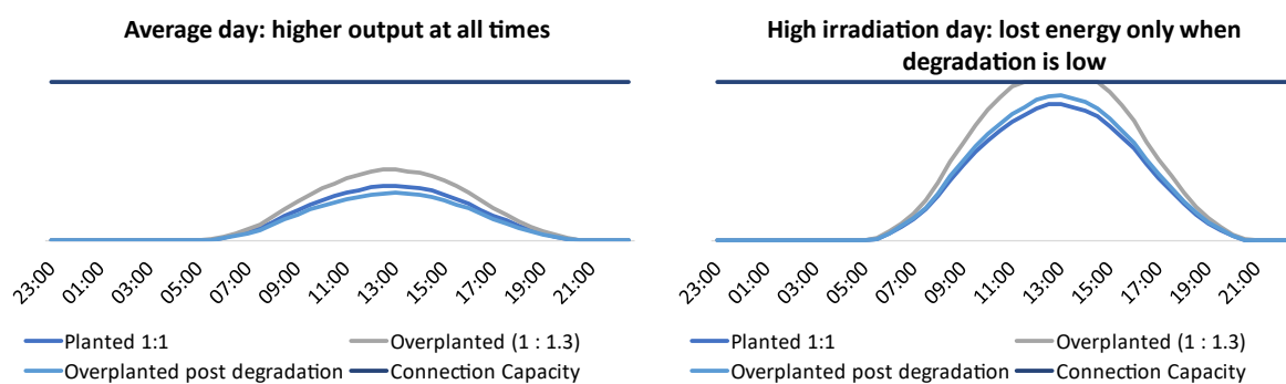
Figure 6-4: Illustrating clipped generation vs. optimised generation on overplanted solar schemes vs. unitary schemes [Author Analysis]
