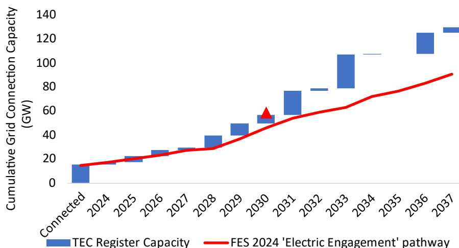
Figure 5-4: Current and potential future connected capacity of offshore wind technology [Ref. 38(2024), Table ES1, Author Analysis]
