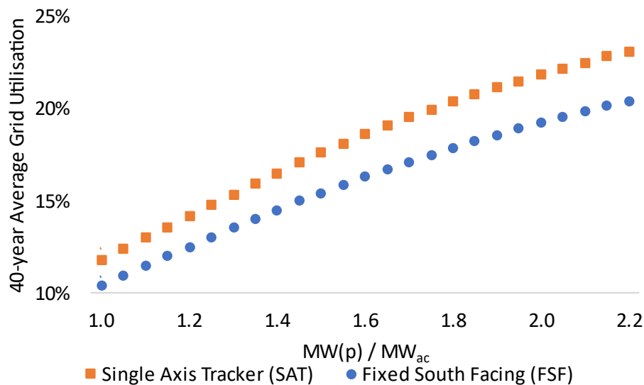
Figure 6-5: Grid Utilisation increases as overplanting increases, but gains are incrementally smaller above a ratio of c.1.5. [Author Analysis]
