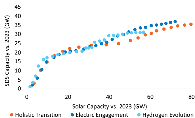
Figure 5-9: Growth in Short Duration Storage capacity vs. Solar Capacity, 2024 – 2050 [Author Analysis, 20(2024), Tables ES.09 & ES1]
