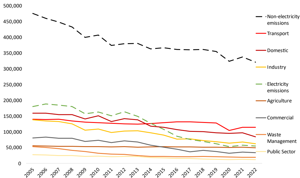
Figure 2-3: National (UK) District GHG Emissions 2005 – 2022 (LULUCF net benefits small and not shown [Ref. 9, Author Analysis])
