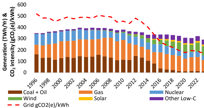
Figure 5-1: Historical Electricity generation (TWh/Yr) and carbon intensity (gCO2(e)/kWh) [Ref. 19, Tables 5.6 & 5.14]
