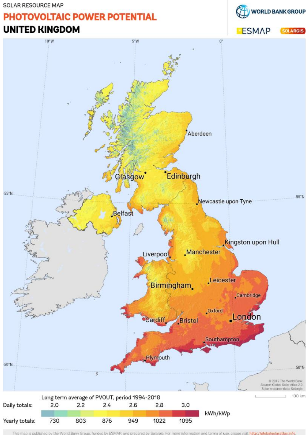
Figure 6-2: United Kingdom solar irradiation [Ref. 68]
