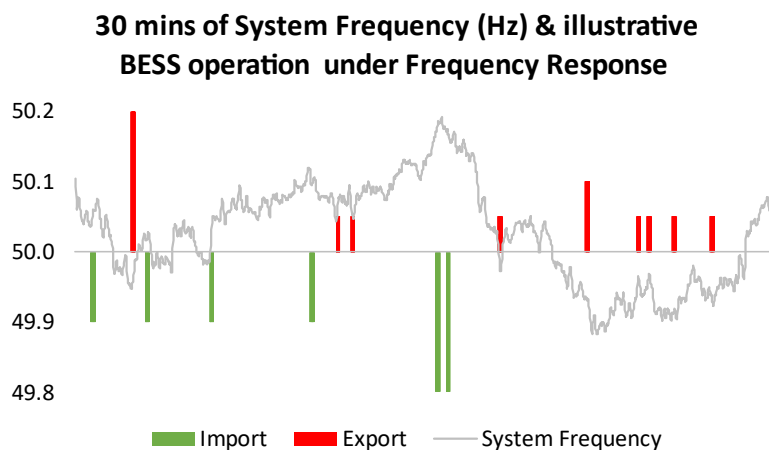
Figure 6-13: 30 mins of system frequency (Hz) and illustrative BESS operation under frequency response [ Author Analysis]
