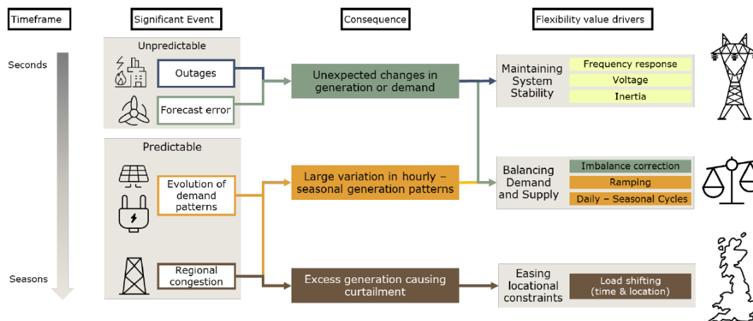
Figure 5-8: Driver of Flexibility Requirements [Ref. 64]
