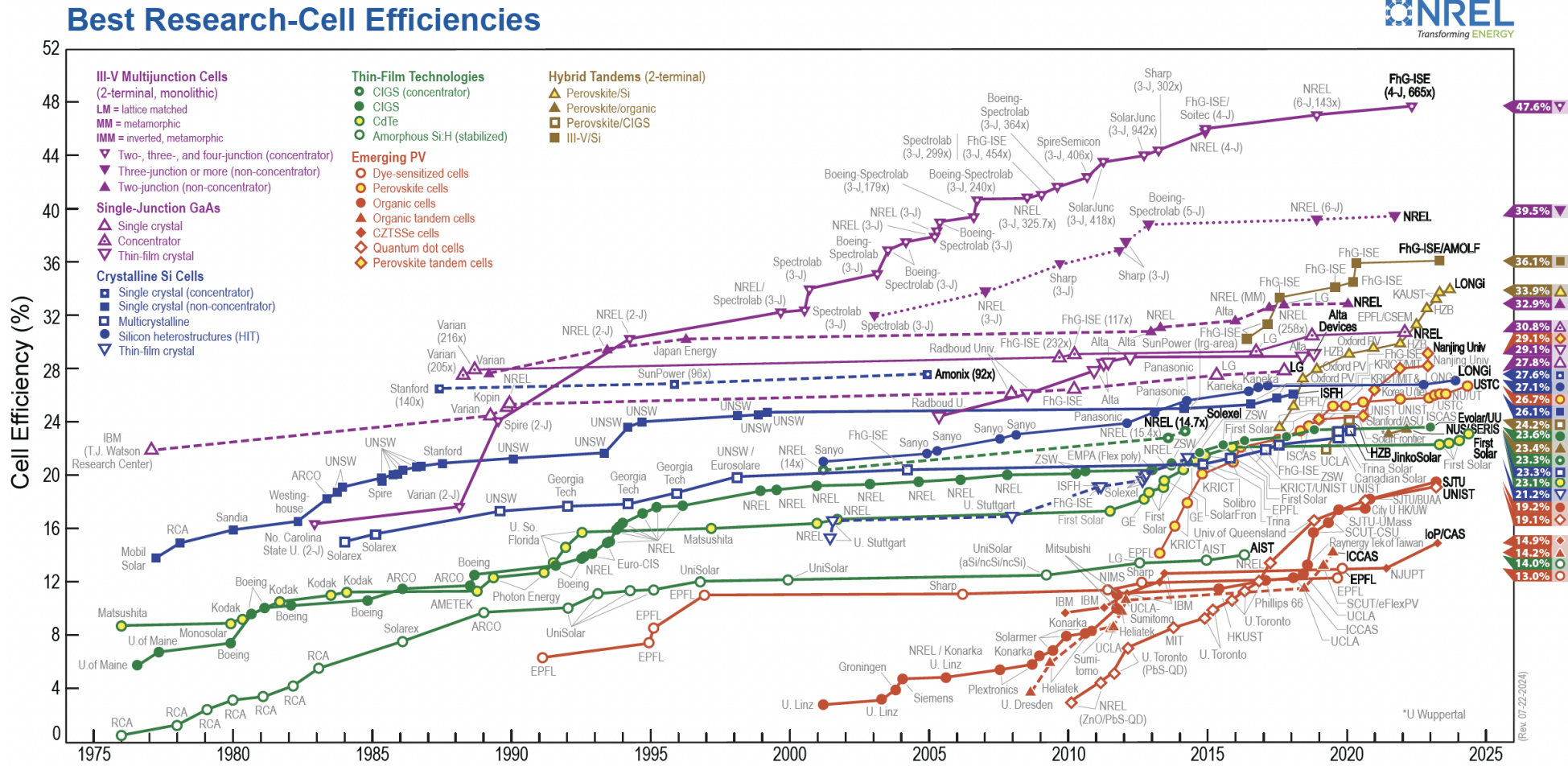
Figure 6-7: Evolution in solar cell efficiency 1975 – 2024 [Ref. 75]
