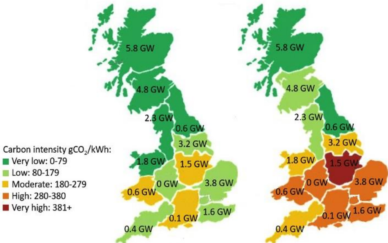
Figure 7-2: NGESO Regional generation carbon intensity analysis (Left: on a higher wind day, Right: on a lower wind day) [Ref. 20(2022)]
