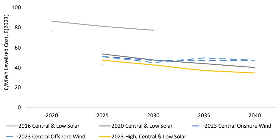
Figure 9-3: Cost of Electricity Generation. An evolution of Levelised Cost forecasts [Ref. 67, Author analysis]
