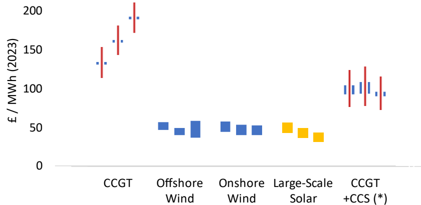
Figure 9-2: Levelised cost of energy comparison [Ref. 67]
