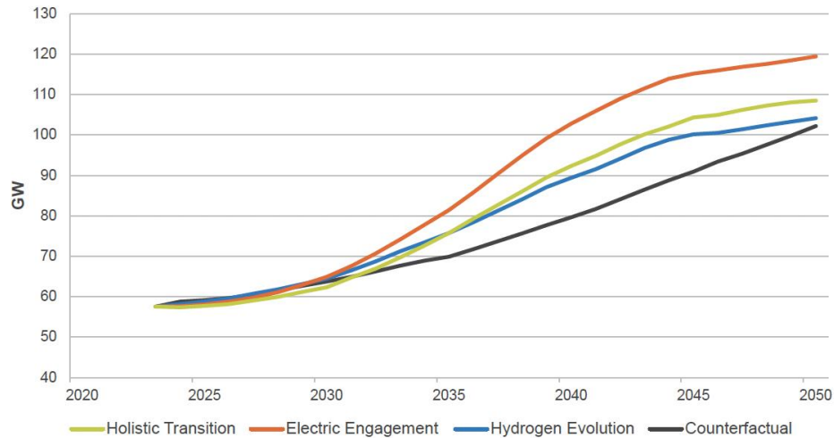
Figure 4-2: Electricity average cold spell peak demand (including losses) [Ref. 19(2024), Figure ES.03]
