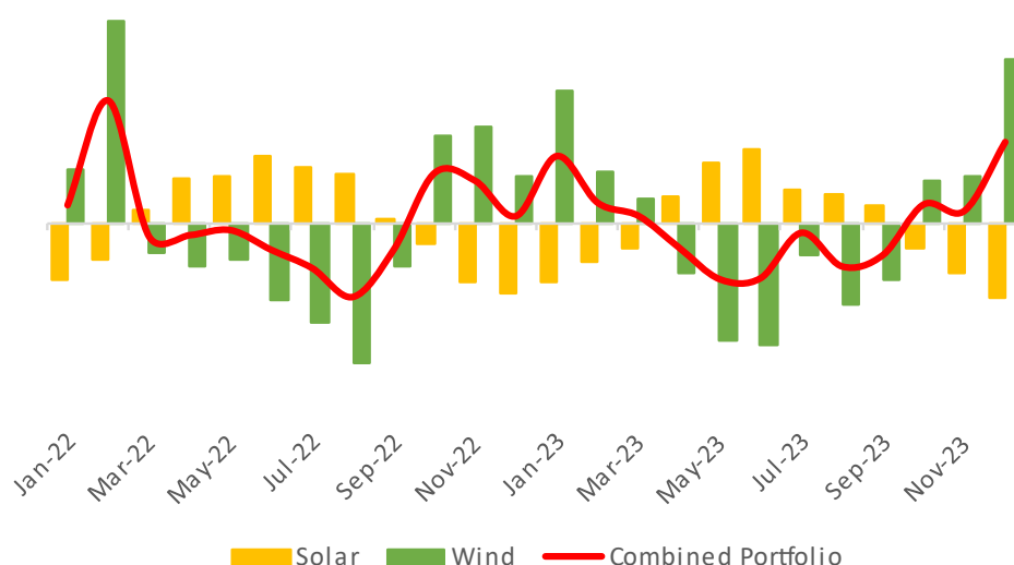
Figure 8-1: Illustrative Generation Dependability for a combined portfolio of solar and wind in GB [Author analysis, Ref. 81, Ref. 20(2024)]
