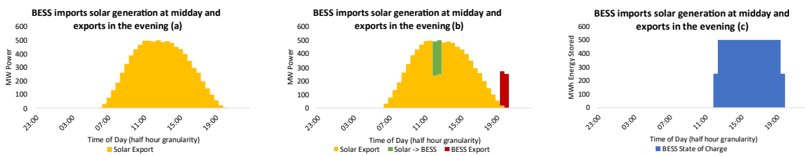
Figure 6-8: BESS imports solar generation at midday and exports in the evening [Author Analysis]
