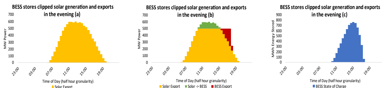
Figure 6-12: BESS stores clipped solar generation and exports in the evening [ Author Analysis]
