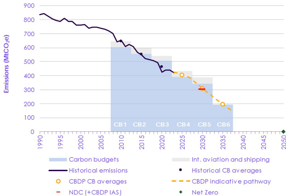
Figure 2-2: UK historical emissions, the CBDP indicative pathway and the UK’s targets [Ref. 8(2024), Figure 1.1]
