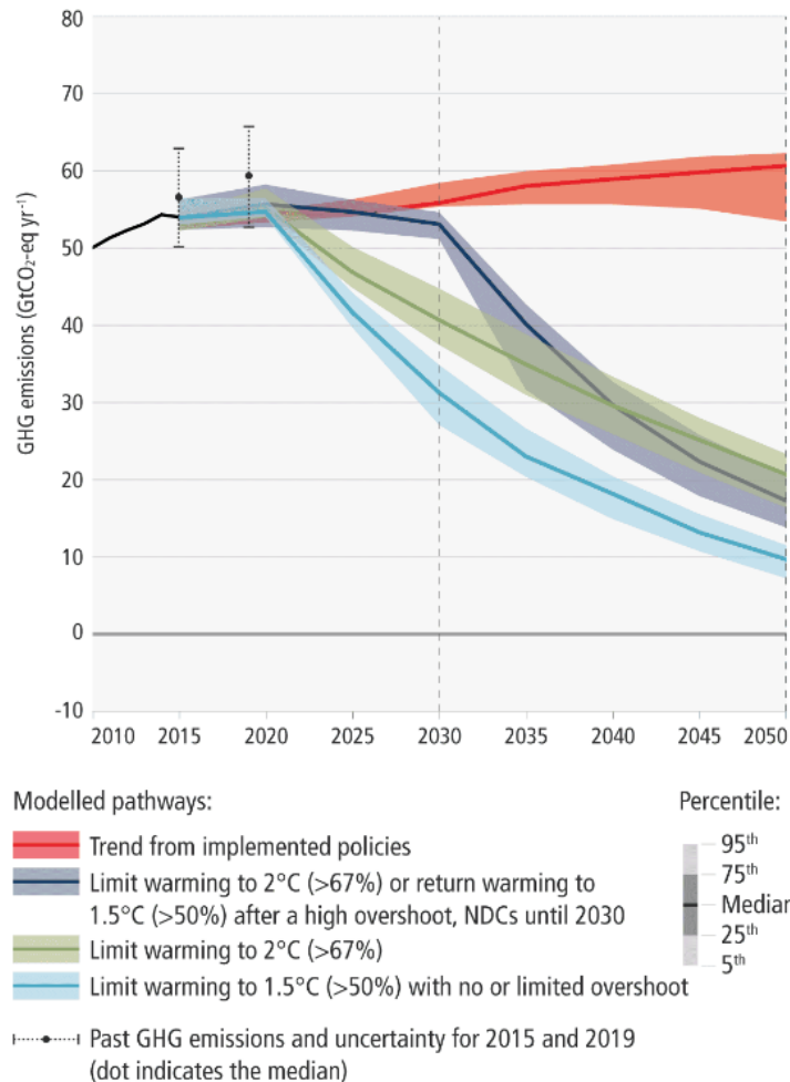
Figure 2-1: Representation of global GHG emissions of modelled pathways [Ref. 3, Figure SPM.4]
