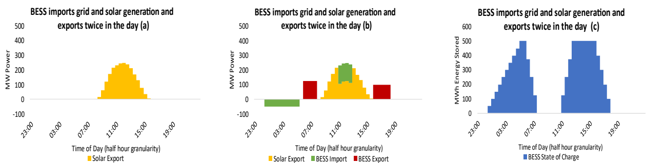
Figure 6-11: BESS imports grid generation and solar generation and exports twice in the day [Author Analysis]
