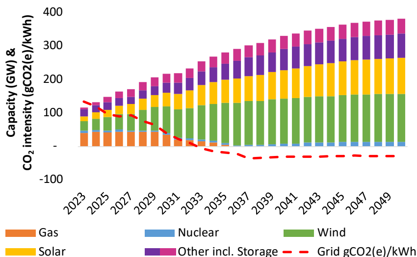
Figure 5-3: Projected electricity generation capacity (GW) and carbon intensity (gCO2(e)/kWh) [Ref. 20(2024), Tables ES.09 & ES1 – ‘System Transformation’]
