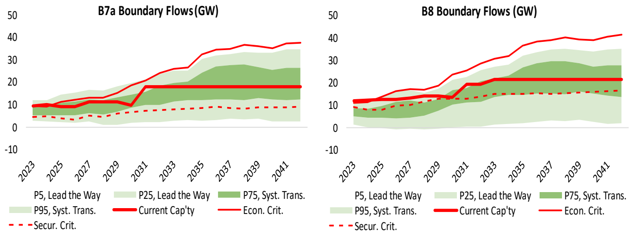
Figure 7-3: B8 and B9 Boundary flows under most extreme scenarios [Ref. 76, Boundary Data workbook]
