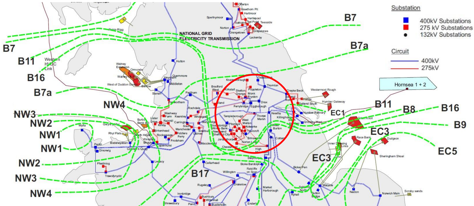
Figure 7-4: Transmission System within 50km of Thorpe Marsh [Ref. 76, Appendix A]
